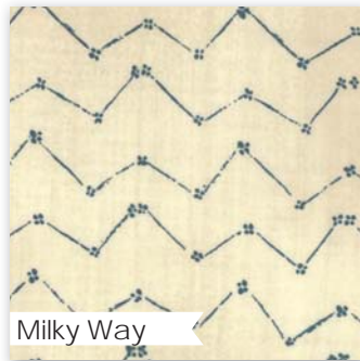
Milky Way
