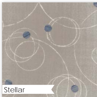
Stellar
