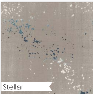
Stellar
