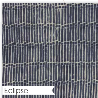
Eclipse
