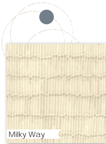
Milky Way
