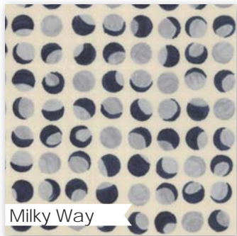
Milky Way
